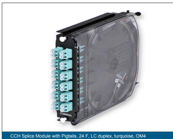
CCH Splice Module with Pigtails, 24 F, LC duplex, turquoise, OM4
