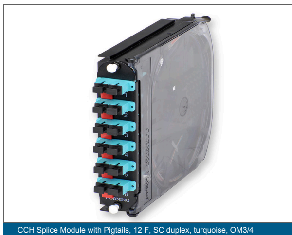
CCH Splice Module with Pigtailed, 12 F, SC duplex, turquoise, OM3/4
